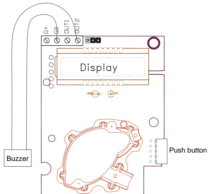
Figure 3 PCB with buzzer connected to OUT2. The push button can be used to silence the buzzer for 30 minutes
