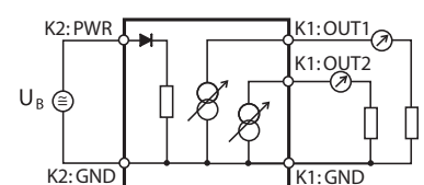
3-wire transmitter current signal
